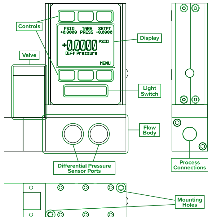
This is a typical differential pressure configuration.
