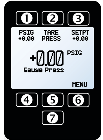
The main display . Note bottom button (7), which toggles the device backlight.
